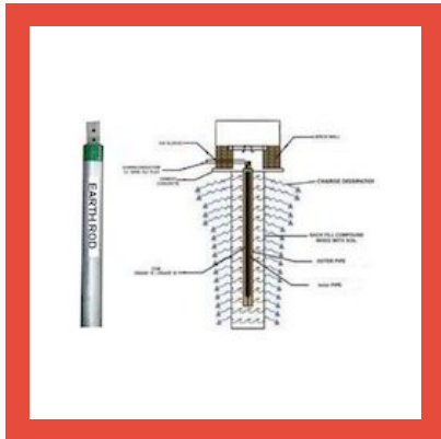
Earthing Rod
