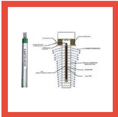
Gel Earthing Electrode
