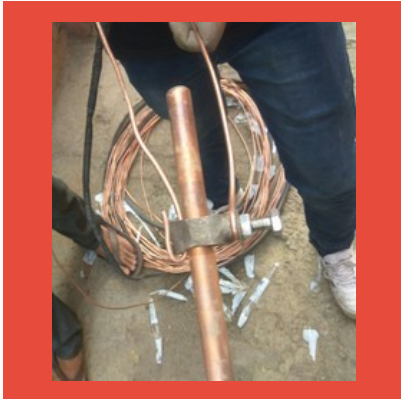
Rod Type Copper Bonded Earthing
