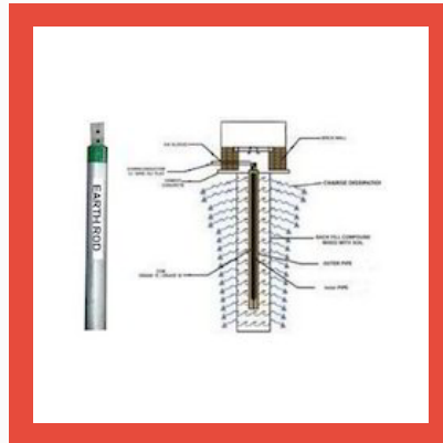
Maintenance Free Earthing
